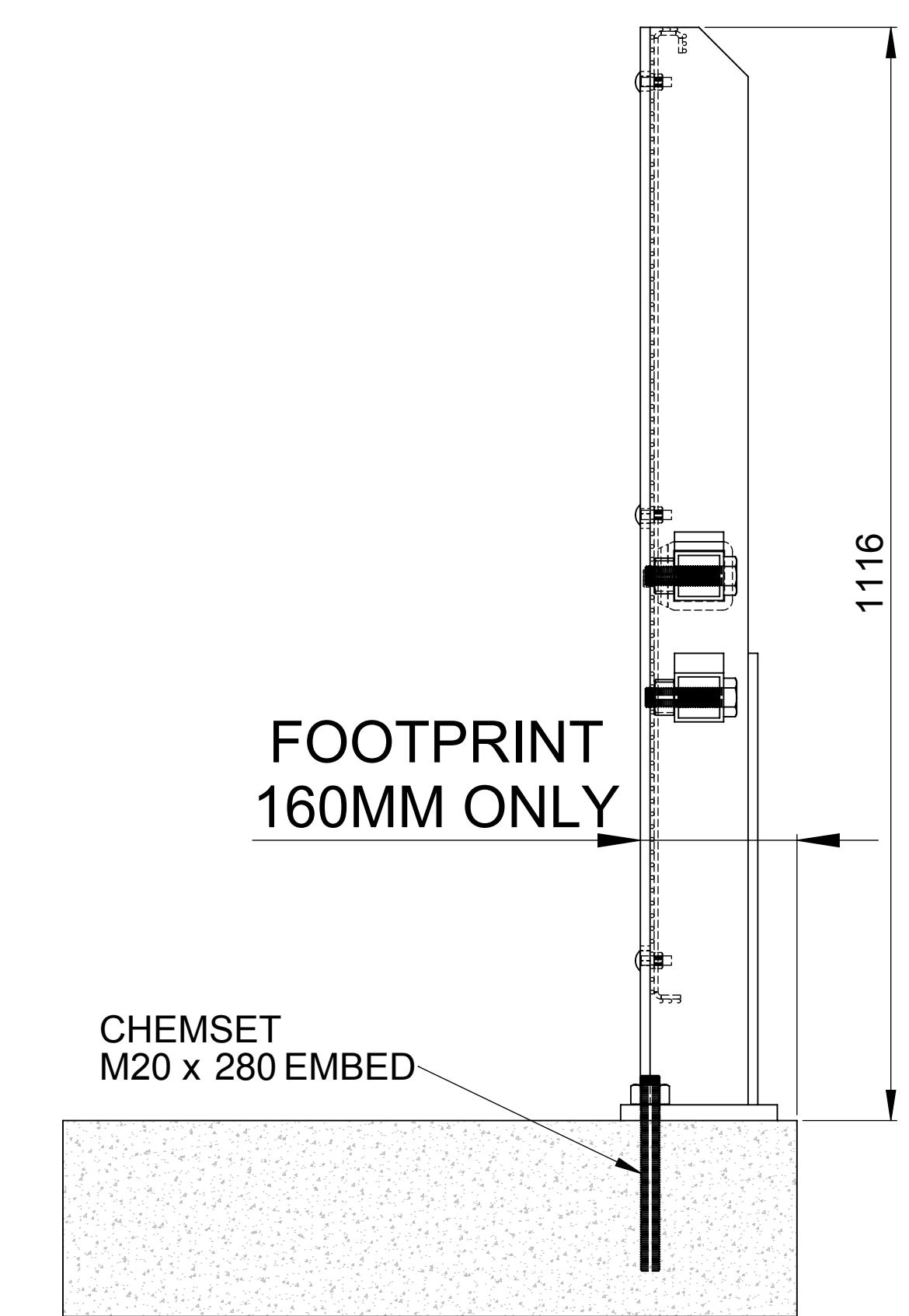
SIDE VIEW
