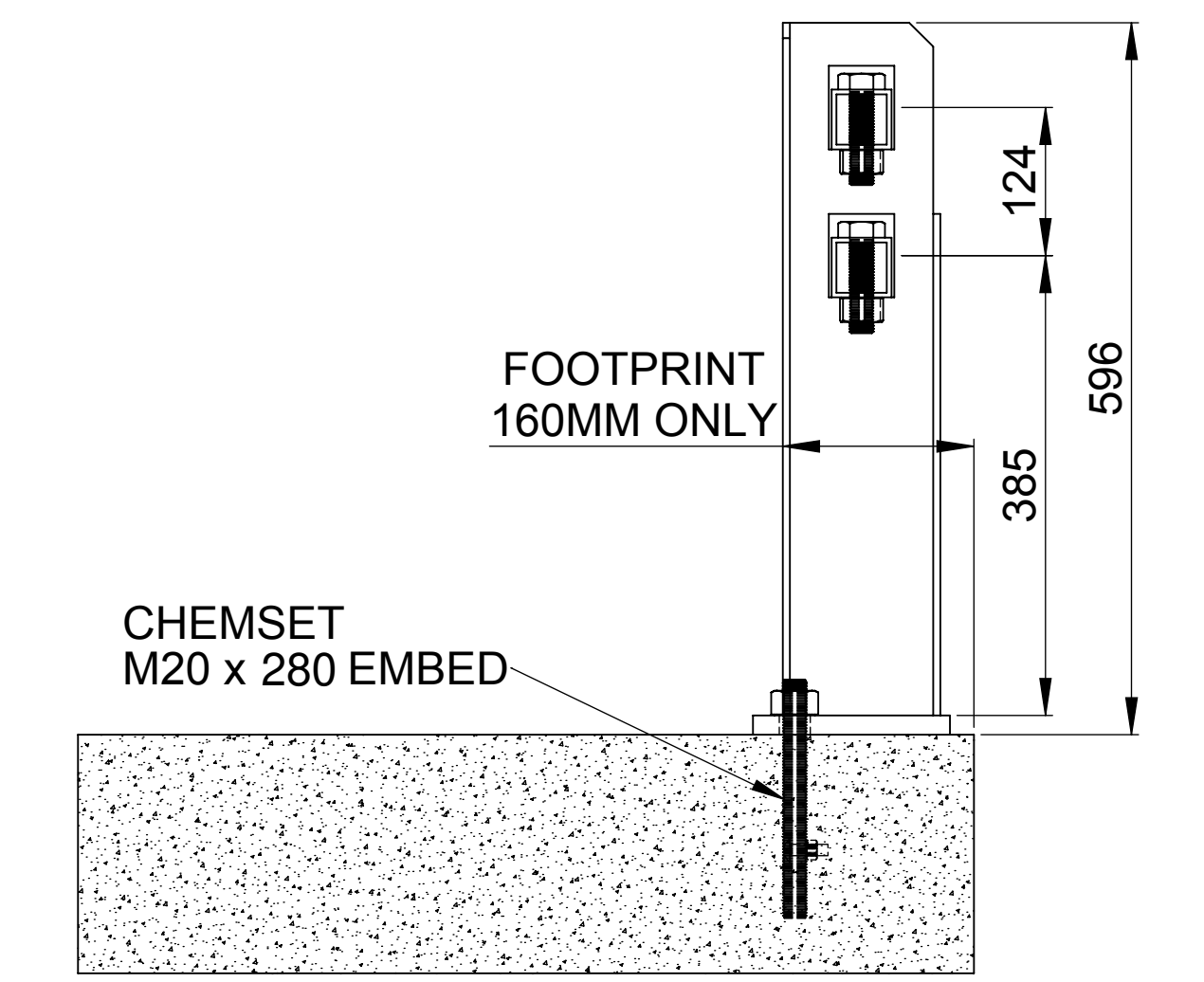
SIDE VIEW
